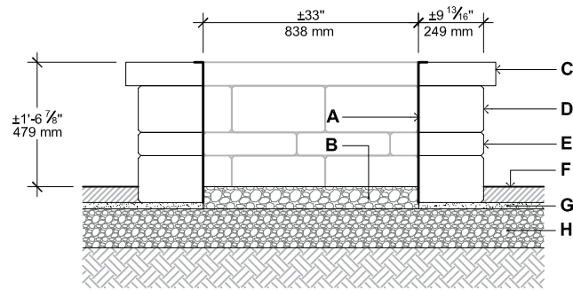
SECTION 1-1
